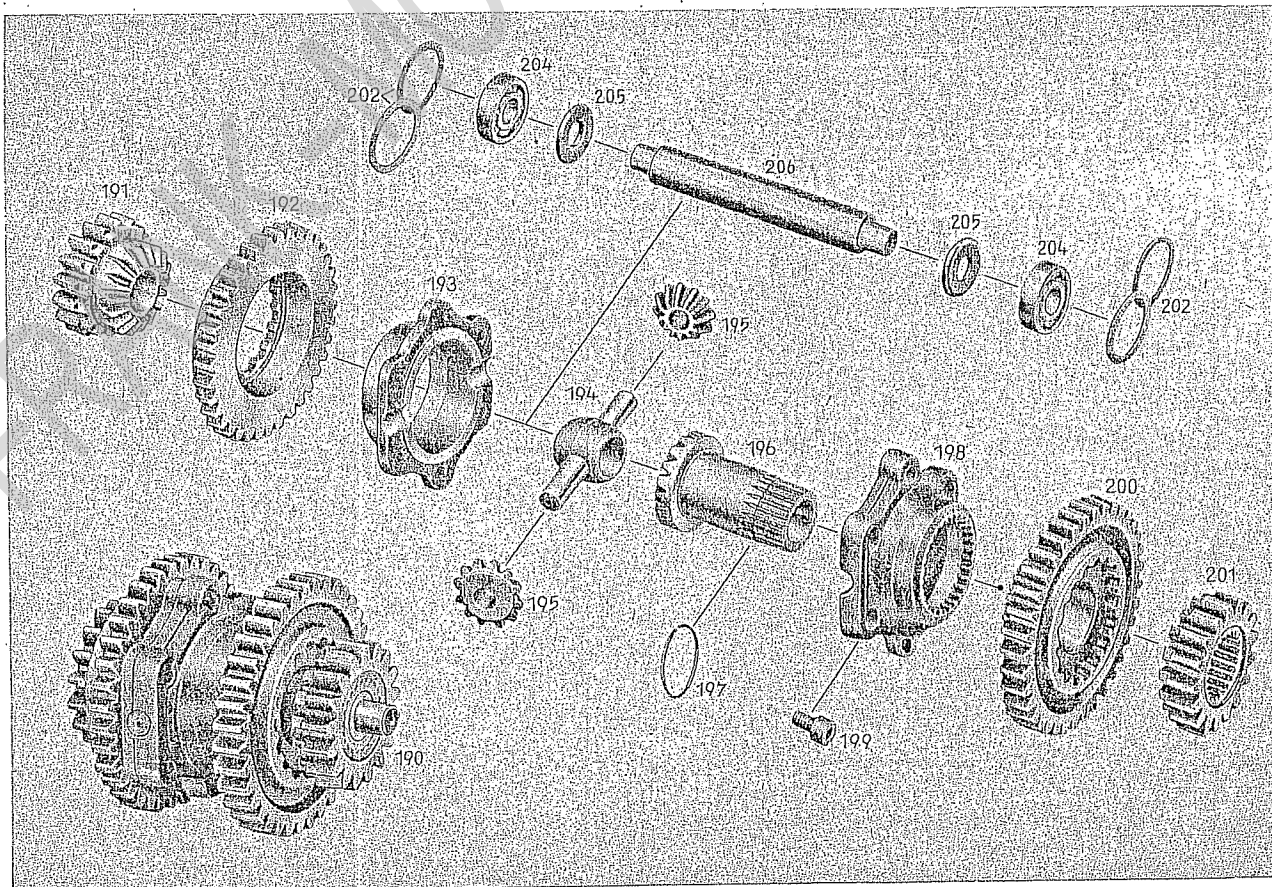
Tafel 3: Differential
